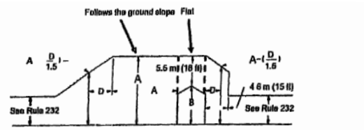
Figure 234-4(b)—Clearance envelope for grain bins filled by portable augers, conveyors, or elevators
