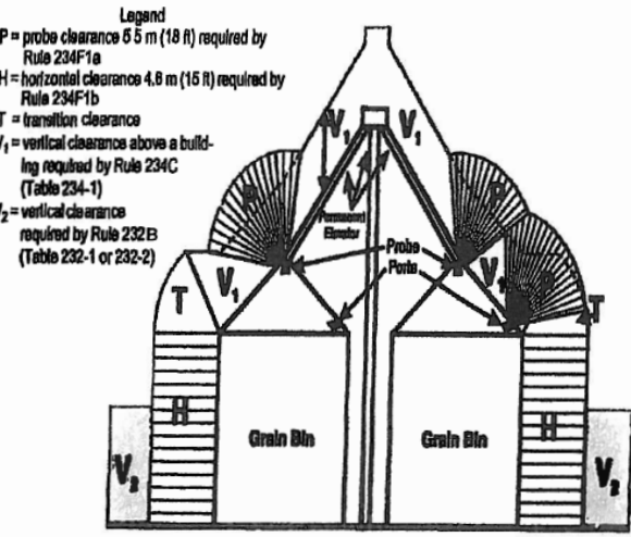
Figure 234-4(a)—Clearance envelope for grain bins filled by permanently installed augers, conveyors, or elevators
